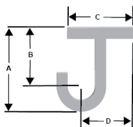
Ceiling Mount Single Bracket Dimensions
