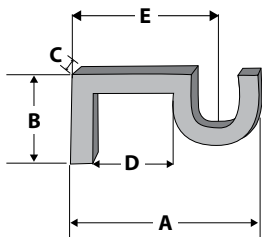
Bracket Dimensions
