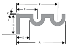
Wall Mount Double Bracket Dimensions
