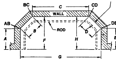
Style 3: For pricing add A, B & C
