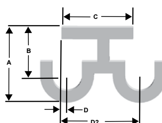
Ceiling Mount Double Bracket Dimensions
