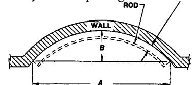
Style 5: For pricing add A & B
