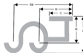
Ceiling Mount Double Bypass Bracket Dimensions
