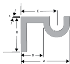
Wall Mount Single Bracket Dimensions
